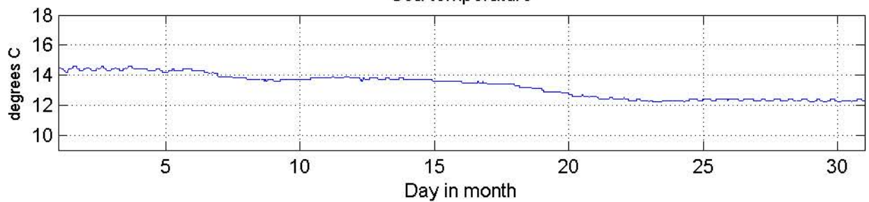
Sea temperature
